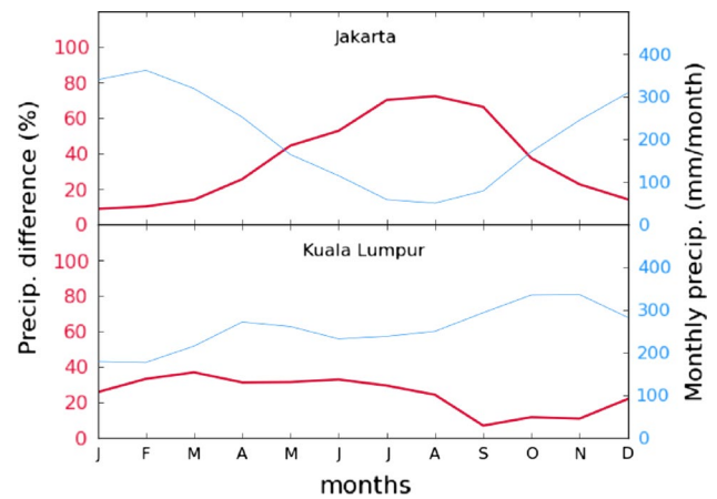
Fig. 8 Seasonal cycle of the difference between WRF2 and WRF2 NoUrb in monthly precipitation (red) and monthly precipitation climatology from WRF2 NoUrb (blue) using a 3-month running average. Results are shown for Jakarta and Kuala Lumpur urban grid points as shown in Fig. 5c, d
