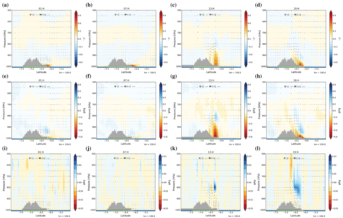
Fig. 10 Vertical profiles of differences over Jakarta between WRF2 and WRF2 NoUrb in temperature (a–d), mixing ratio (e–h) and cloud mixing ratio (i–l). Vectors indicate differences in winds along the vertical
