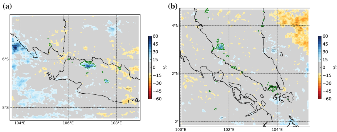
Fig. 7 Difference between WRF2 and WRF2 NoUrb in total precipitation in Java domain (a) and Malay Peninsula domain (b). Stippling indicates that differences are statistically significant using a Wilcoxon
