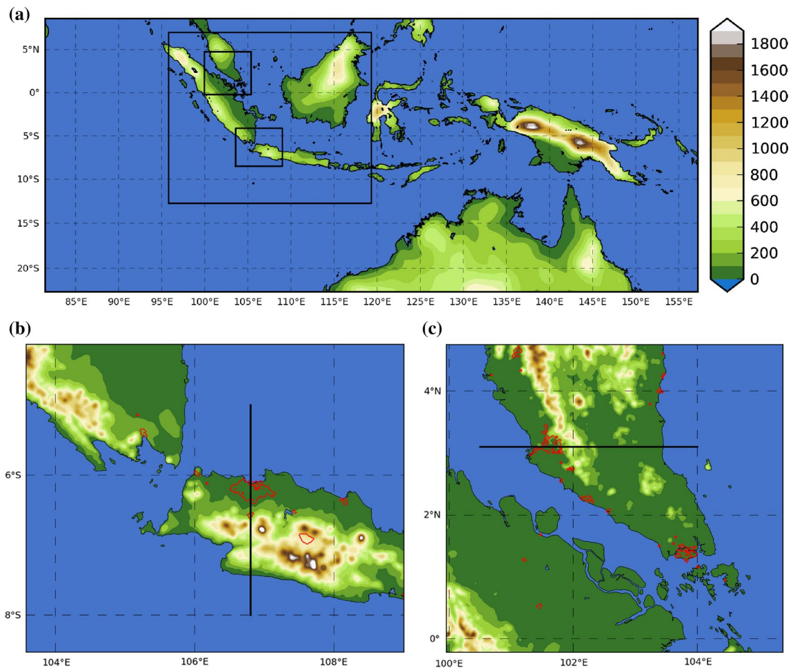
Fig. 1 Model domains and topography. a Outer domain spans the entire map and nested domains are delimited by black rectangles . b Domain 3 centred in West Java and c domain 4 centred in Southern
