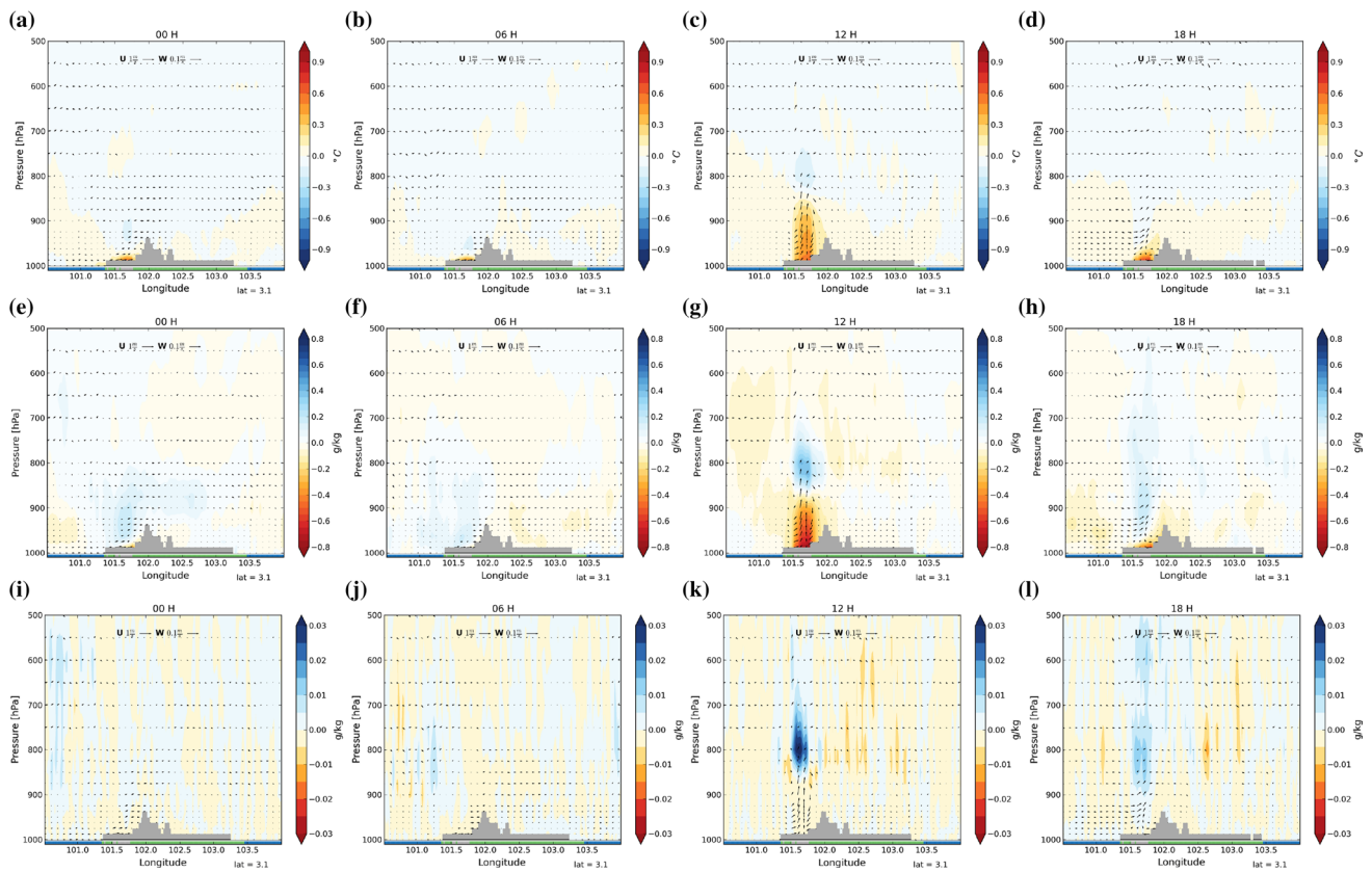
Fig. 11 As Fig. 10 but over Kuala Lumpur
