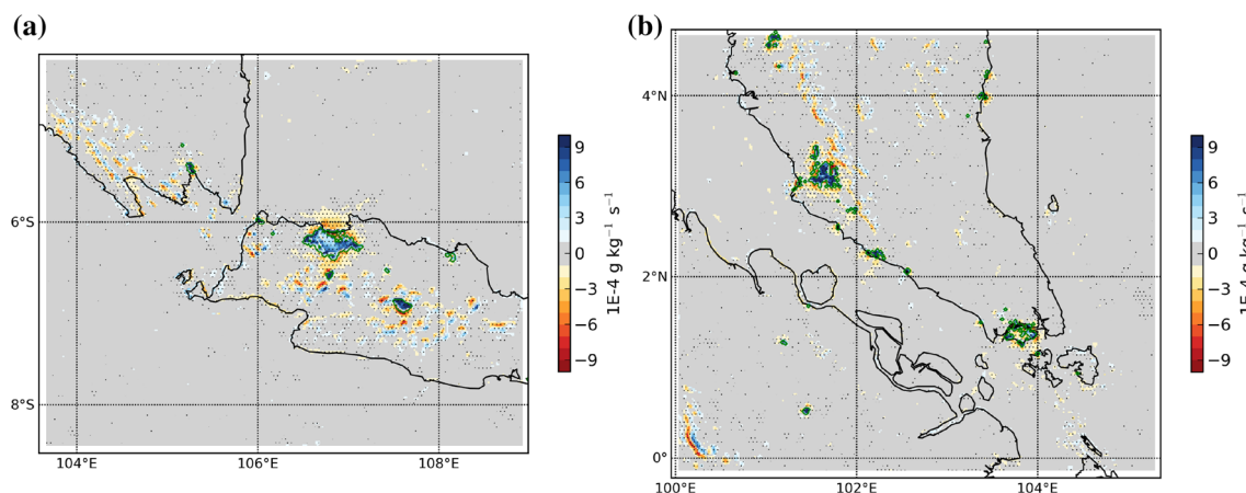
Fig. 9 Difference between WRF2 and WRF2 NoUrb in moisture flux convergence in Java domain (a) and Malay Peninsula domain (b). Stippling indicates that differences are statistically significant using a
