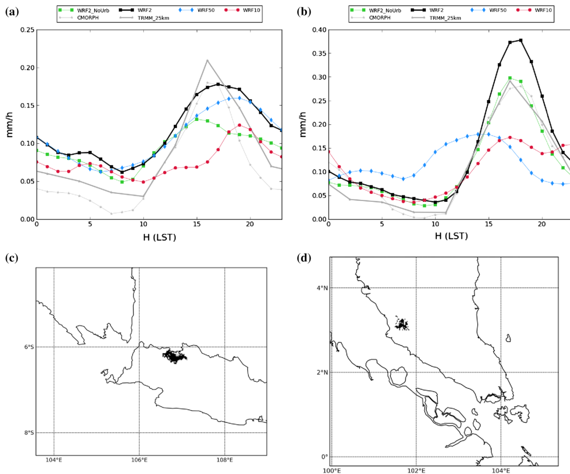
Fig. 5 Diurnal cycle of precipitation over Jakarta (a) and Kuala Lumpur (b) urban grid points for the different datasets. Urban points are marked with black areas in c and d
